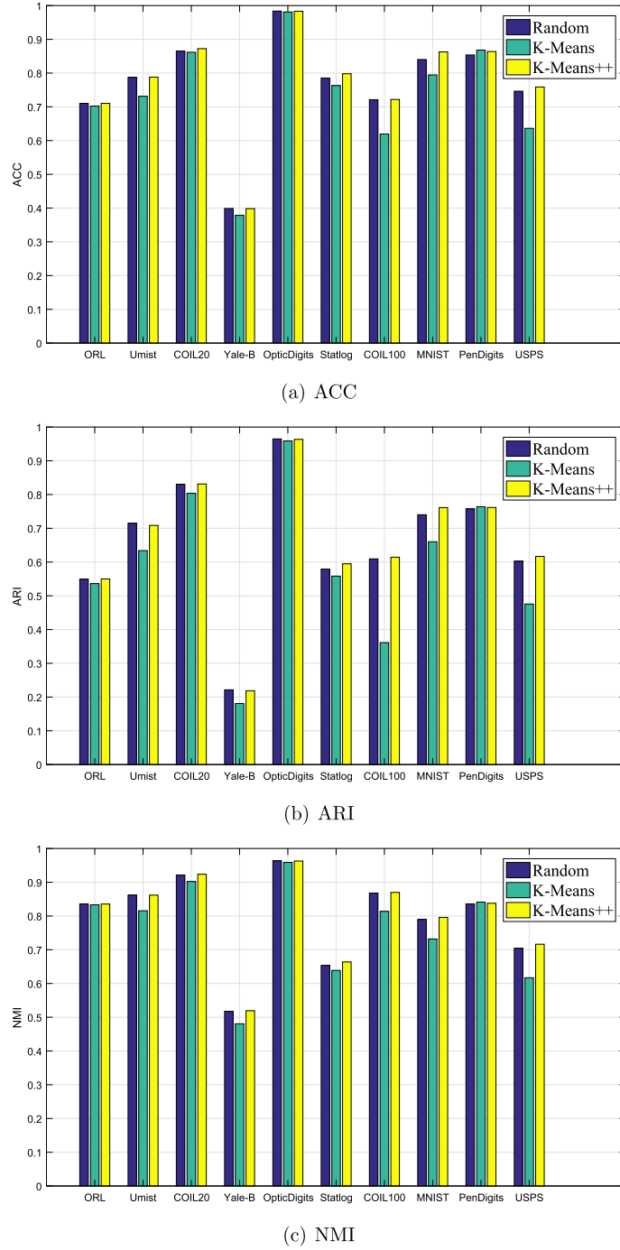
Fig. 8. Comparison of different initialization for Y .
