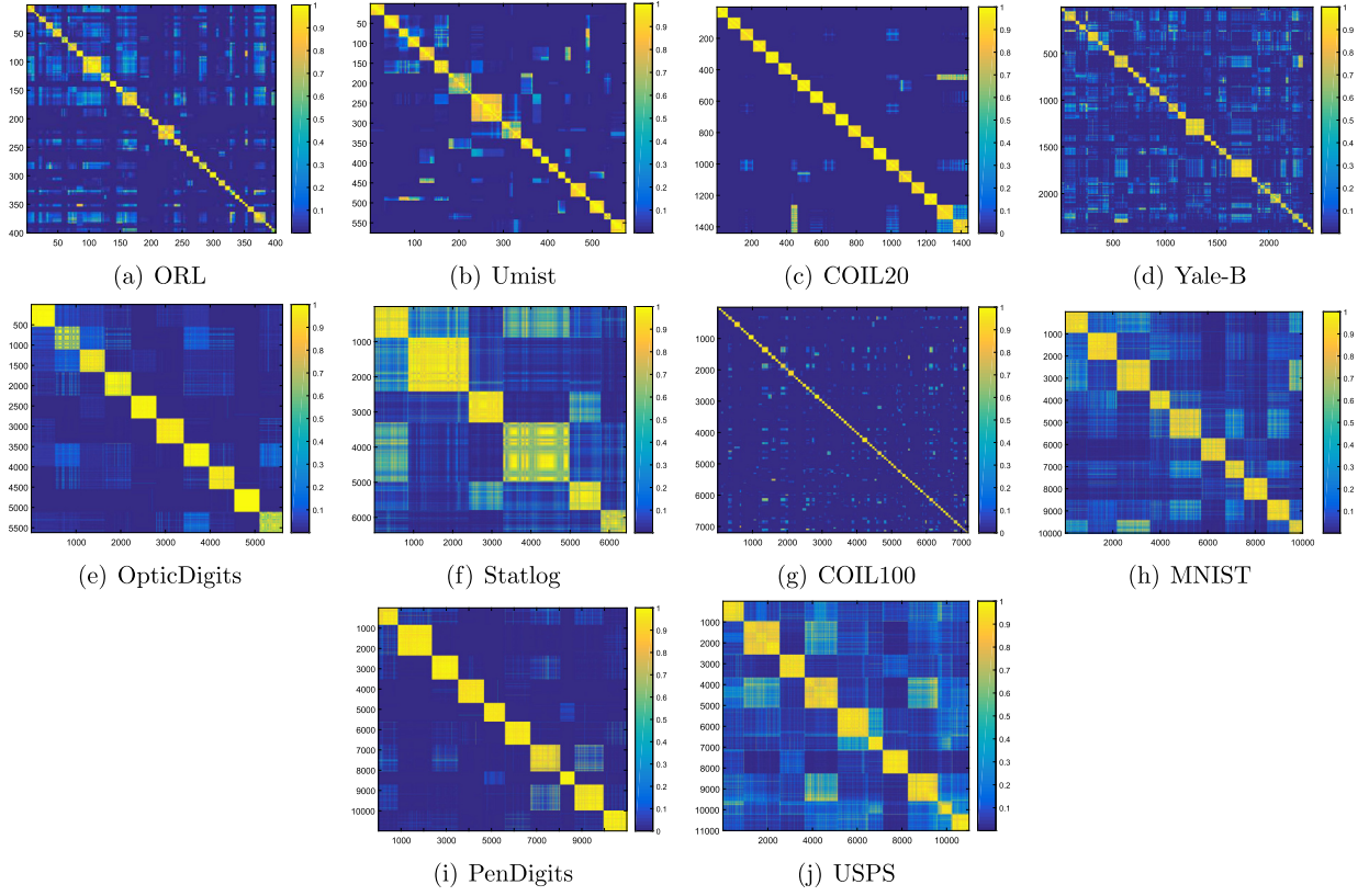
Fig. 10. Evaluation of the learned constraints.
