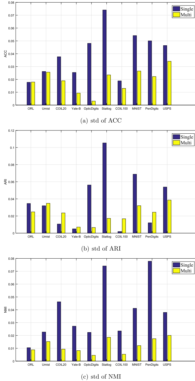
Fig. 6. Comparison of robustness between single and multiple constraints.
